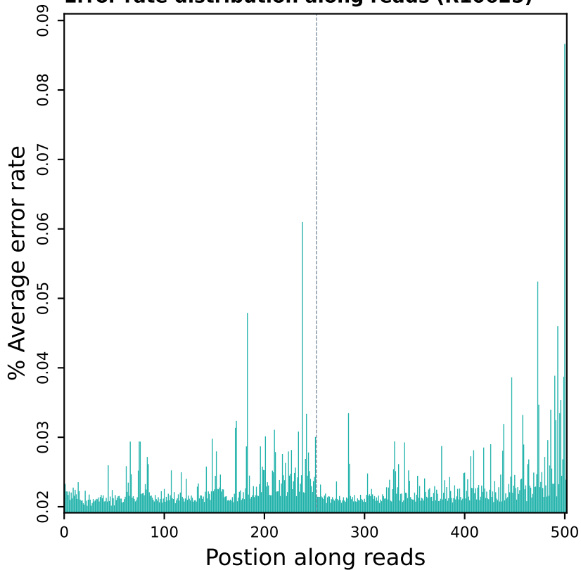
Error rate distribution along reads (R10625)
